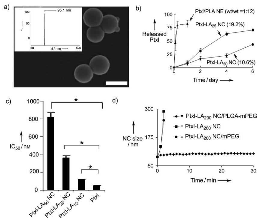
Figure 2. Characterization and properties of Ptxl–PLA NCs. a) Ptxl–LA 25 (paclitaxel–PLA NC prepared at a LA/Ptxl ratio of 25:1) analyzed by scanning electron microscopy (SEM) and dynamic light scattering (DLS, inset). Scale bar = 150 nm. b) Release kinetics of Ptxl from Ptxl–PLA NCs and Ptxl–PLA NE (prepared by nanoprecipitating a mixture of Ptxl and PLA (Ptxl/PLA (wt/wt) = 1:12) at 37°C in 1 × PBS. c) Toxicity evaluation of Ptxl–LA 50 NC, Ptxl–LA 25 NC, Ptxl–LA 10 NC, and Ptxl using MTT assay in PC-3 cells after incubation for 24 h. Significance at 95 % confidence interval is marked with an asterisk (*). d) Stability of Ptxl–LA 200 NC in PBS at 37°C before and after being treated with PLGA–mPEG 5k or mPEG 5k .
