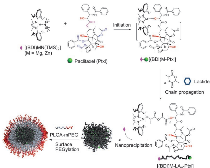
Figure 1. Preparation of poly(ethyleneglycol)ated (PEGylated) Ptxl–PLA NCs by means of Ptxl-initiated LA polymerization in the presence of [(BDI)MN(TMS)_2] ( M = Mg, Zn ), followed by nanoprecipitation and noncovalent surface modification with poly(glycolide-co-lactide)- b -methoxylated PEG (PLGA-mPEG) (PLGA-mPEG).
